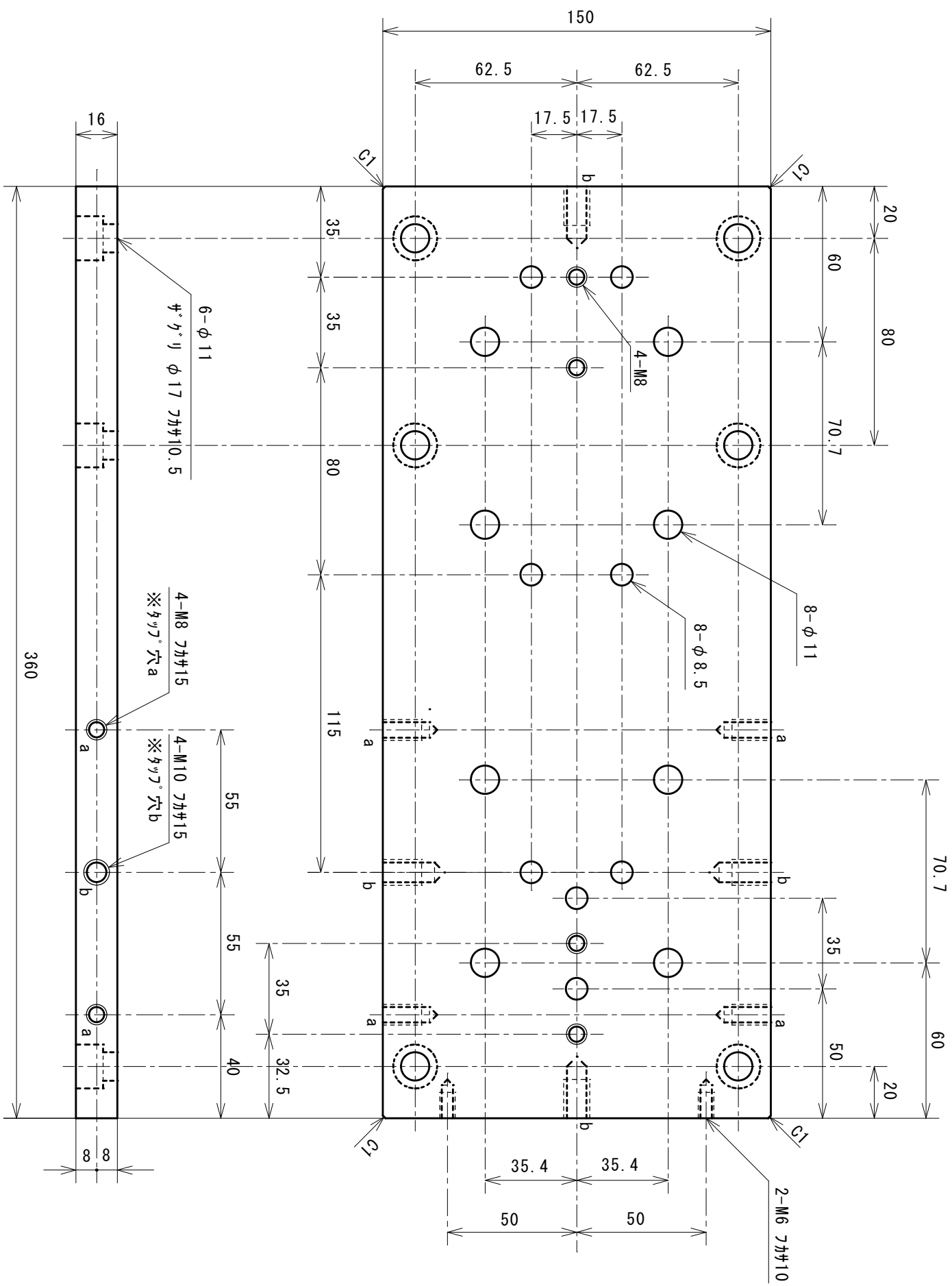
WC Plate For Melion-250CRS
